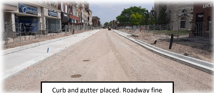
Curb and gutter placed. Roadway fine graded and ready for base asphalt
